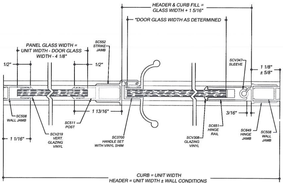
HORIZONTAL CROSS SECTION
